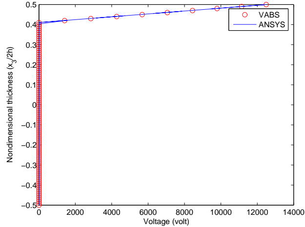
Fig. 3. Voltage variation along the thickness
