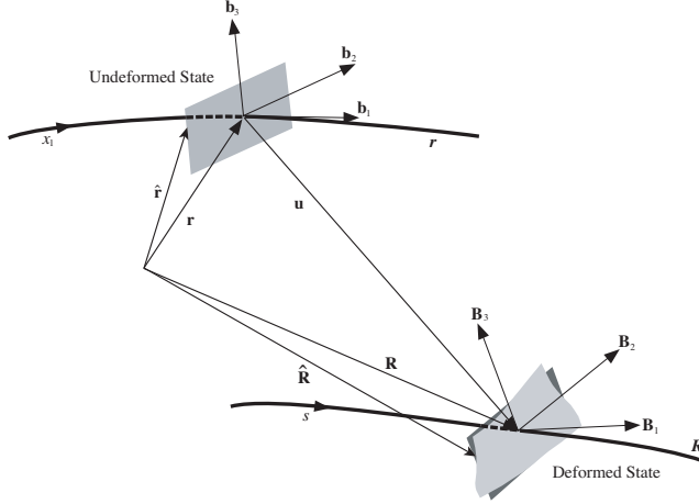
Fig. 1. Schematic of beam deformation
