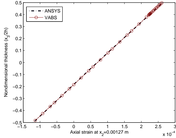
Fig. 5. Axial strain variation at x_1 = 0.5l
